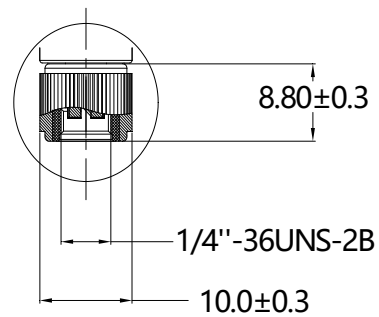
RF SMA-Male DETAIL A SCALE 2:1
