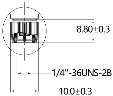
SMA-Male DETAIL A SCALE 2:1
