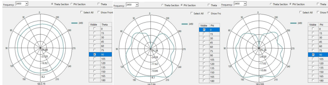
2D Radiation Pattern at 2450MHz
